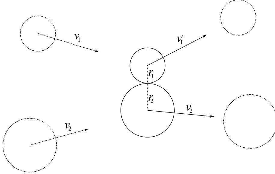
Figure 3: Collision between two particles.
