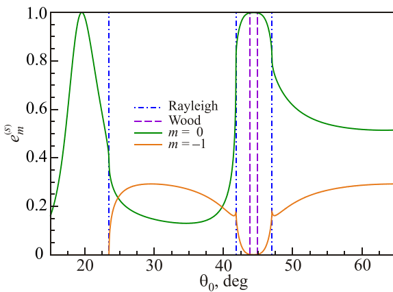
FIG. 6. The diffraction efficiencies in reflection e_m^{(s)} as functions of the angle of incidence \theta_0 . The vacuum wavelength of the incident light is \lambda/a = 2.0972 [ \omega_R a/c\pi = 0.9536 ], and is indicated by the triangle on the dispersion curve in Fig. 2(a) at ka/\pi = 0.9896 . Rayleigh anomalies are expected for angles of incidence \theta_0^R = \pm 23.46^\circ , \pm 41.81^\circ and \pm 47.01^\circ (dash-dotted lines). Wood anomalies are predicted from Eq. (15) to occur at angles of incidence \theta_0^W = \pm 43.77^\circ and \pm 44.94^\circ (dashed lines).
