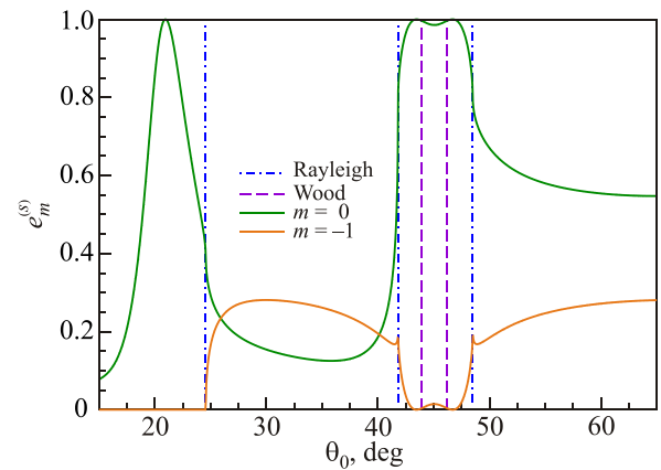
FIG. 4. The diffraction efficiencies in reflection e_m^{(s)} as functions of the angle of incidence \theta_0 . The vacuum wavelength of the incident light is \lambda/a = 2.1236 [ \omega_R a/c\pi = 0.9418 ], and is indicated by the square on the dispersion curve in Fig. 2(a) at ka/\pi = 0.9798 . Rayleigh anomalies are expected at angles of incidence \theta_0^R = \pm 24.57^\circ , \pm 41.81^\circ and \pm 48.51^\circ (dash-dotted lines). Wood anomalies are predicted from Eq. (15) to occur at angles of incidence \theta_0^W = \pm 43.91^\circ and \pm 46.23^\circ (dashed lines).
