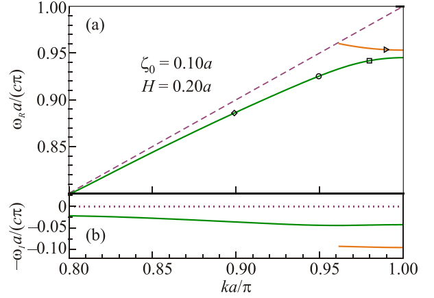
FIG. 2. The (a) real part \omega_R(k) and (b) the imaginary part \omega_I(k) of the complex frequency \omega(k) = \omega_R(k) - i\omega_I(k) of the leaky surface electromagnetic wave supported by the structure depicted in Fig. 1. The values of the parameters defining this structure are \epsilon_1 = 2.25 , \epsilon_2 = 15 , and \epsilon_3 = 1 . The surface profile function is \zeta(x_1) = \zeta_0 \cos(2\pi x_1/a) [Eq. (12)], with \zeta_0/a = 0.10 and H/a = 0.20 . A 31 \times 31 matrix system (i.e., N = 15 ) was used to obtain these results. The vacuum light line is indicated by a dashed line in panel (a). The open symbols in panel (a) indicate some frequencies that are discussed in the main text.
