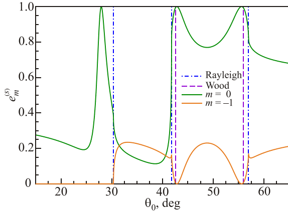
FIG. 5. The diffraction efficiencies in reflection e_m^{(s)} as functions of the angle of incidence \theta_0 . The vacuum wavelength of the incident light is \lambda/a = 2.2578 [ \omega_R a/c\pi = 0.8858 ], and is indicated by the diamond on the dispersion curve in Fig. 2(a) at ka/\pi = 0.8990 . Rayleigh anomalies are expected for angles of incidence \theta_0^R = \pm 30.34^\circ , \pm 41.81^\circ and \pm 56.98^\circ (dash-dotted lines). Wood anomalies are predicted from Eq. (15) to occur at angles of incidence \theta_0^W = \pm 42.58^\circ and \pm 55.96^\circ (dashed lines).
