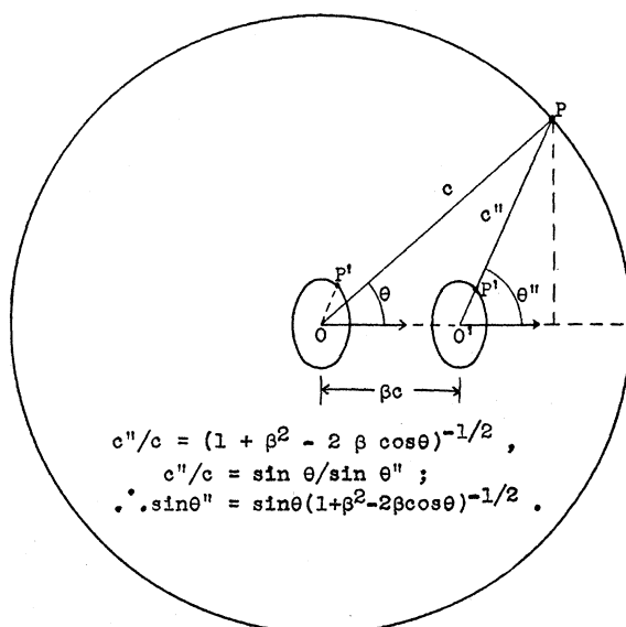
Fig. 3. The ray traversing the moving spheroid at P' at an angle \theta'' reaches the stationary spherical surface drawn about O , at the point P , at an angle \theta .
