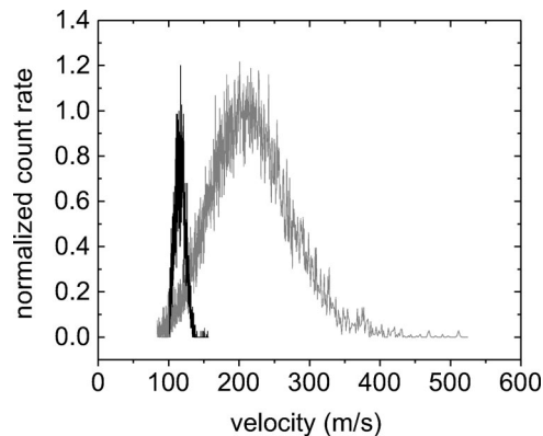
Fig. 5. Velocity distribution of the \text{C}_{60} molecules for a thermal and a velocity selected beam. The thermal beam (gray curve) is centered around v = 200\text{ m/s} and has a width of \Delta v/v \sim 0.6 , while the selected beam (black curve) is centered around \bar{v} = 117\text{ m/s} with a width of \Delta v/v \sim 0.17 . We therefore expect the velocity selected interference pattern to be expanded by 70% on the screen and to show at least three times ( \approx 0.6/0.17 ) as many interference orders as the unselected pattern.
