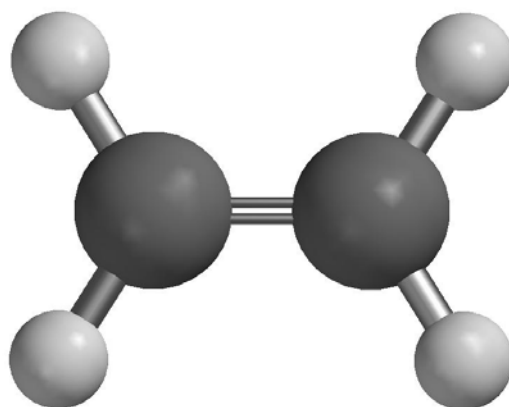
Figure 1. Ethene, C_2H_4
