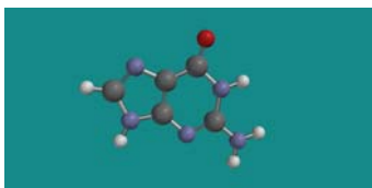
Guanine
