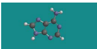
Adenine
