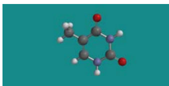
Thymine
