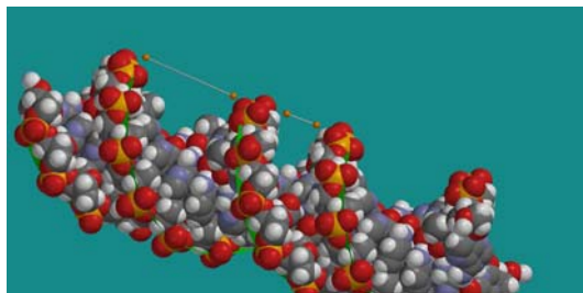
B-DNA: Two grooves of width 12 and 4 Å
